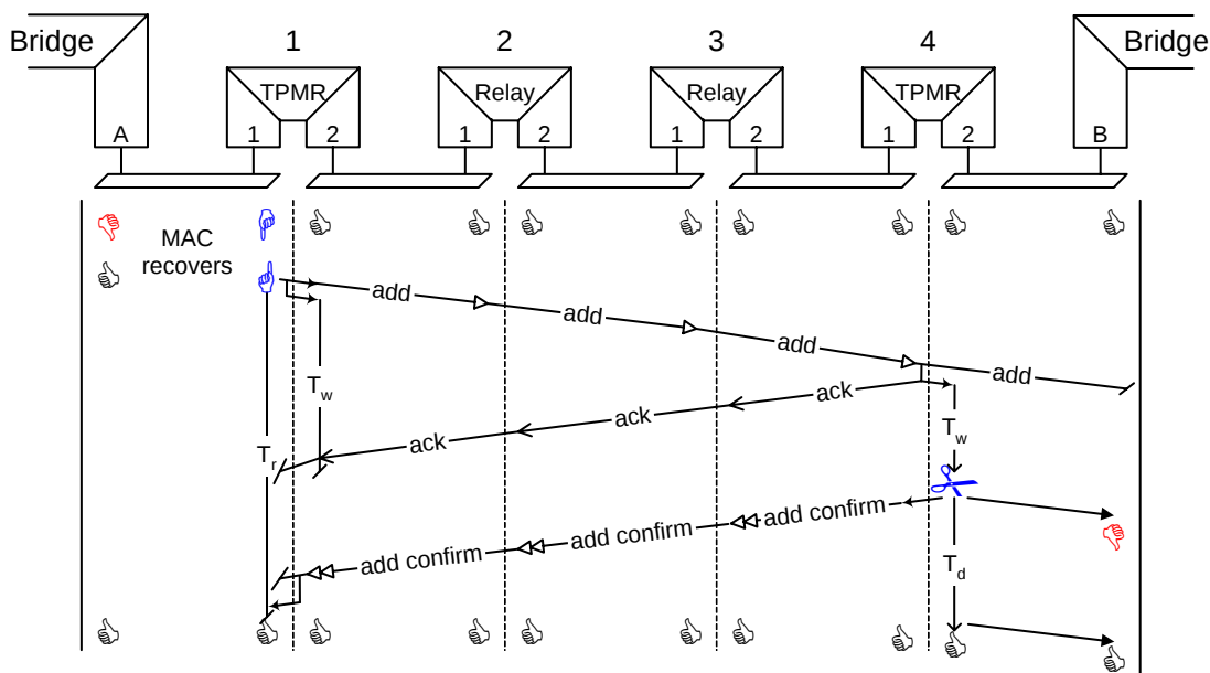
Figure 7—Notification from one end of the link to the other
