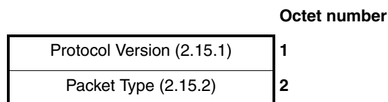
Figure 12—MSPDU structure
