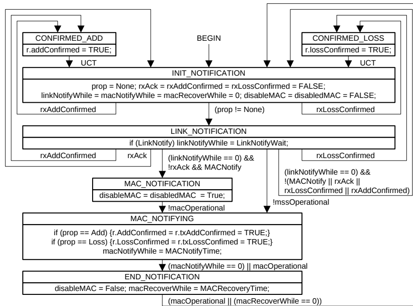
Figure 11—Status Notification state machine
