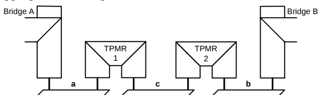
Figure 2—TPMR chain connecting Bridge Ports
