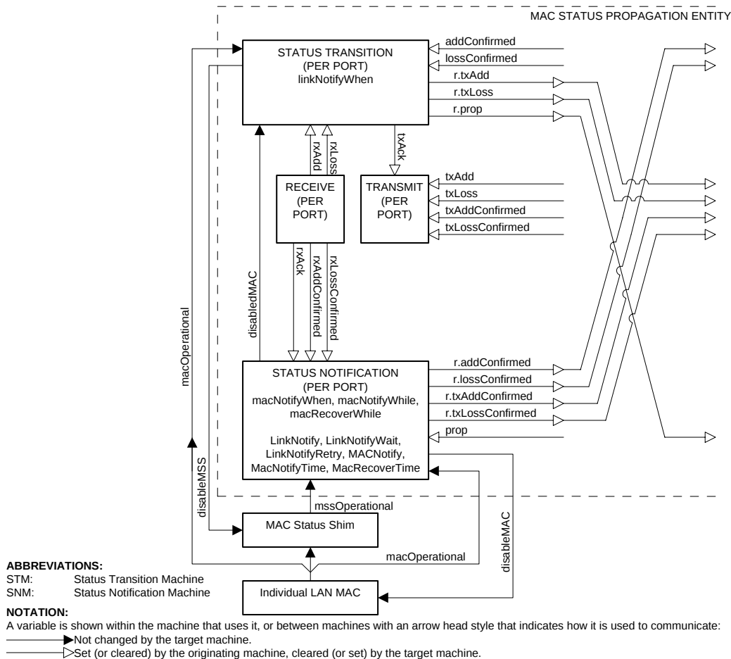
Figure 9—MSPE machine overview
