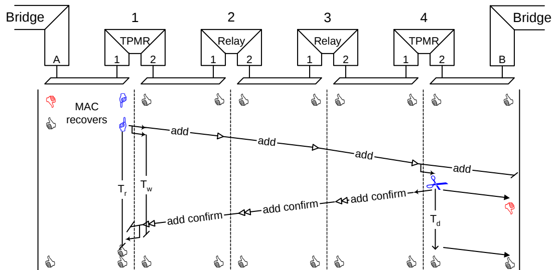
Figure 8—Immediate MAC status notification at the end of a link
