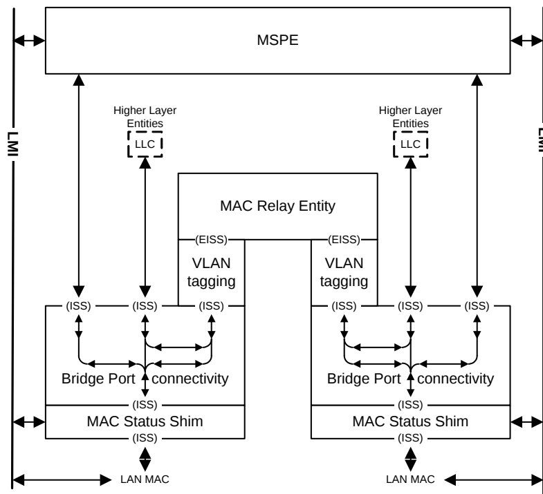
Figure 3—MAC Status Shims and the MAC Status Propagation Entity
